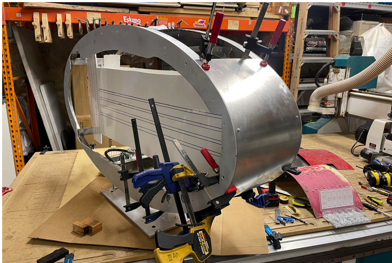
ARK: Caspian Bistro Custom Sign Featuring Retrofitting Old Sign Frame, Fabricating New Face and Return Panels and Installing LED Mounting Panels
